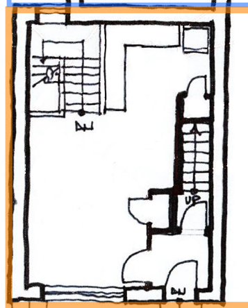
1ST FLOOR
